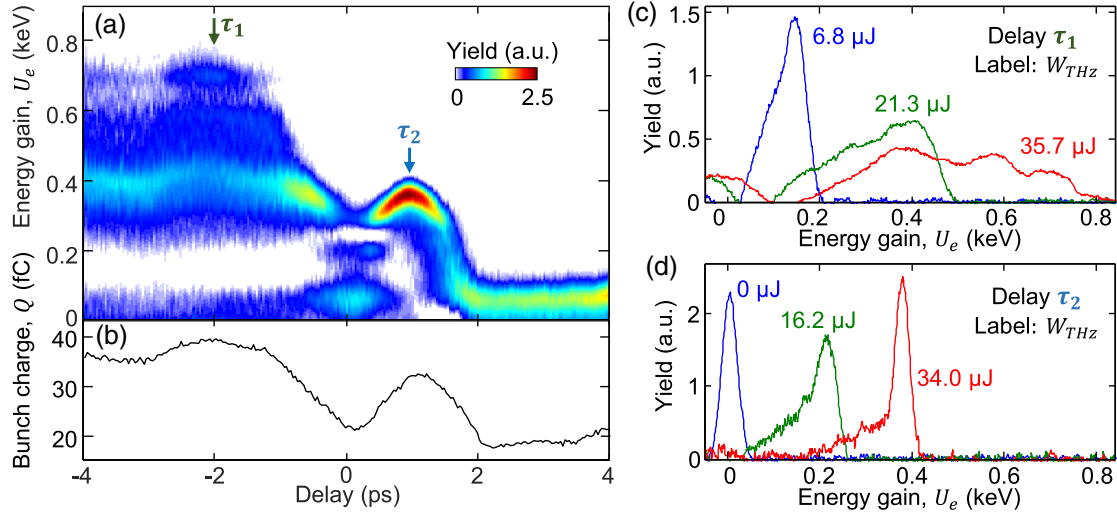
Fig. 3. THz-driven electron energy gain and bunch charge modulation. (a) Measured spectrogram showing the energy gain spectra as a function of delay between UV and THz pulses, at maximum THz energy; (b) measured bunch charge as a function of delay; (c) and (d) electron energy spectra for three different THz energies at delay positions (c) \tau_1 = -2 ps and (d) \tau_2 = 0.9 ps.
